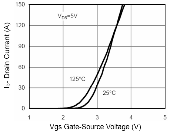
Transfer Characteristic
